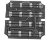
LED unit 16x 1W white + warm white Art. nr.1343101
